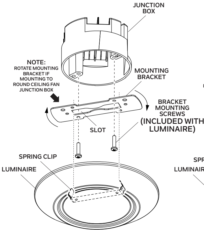
Fig. 2 INSTALLING TO ROUND CEILING FAN JUNCTION BOX
