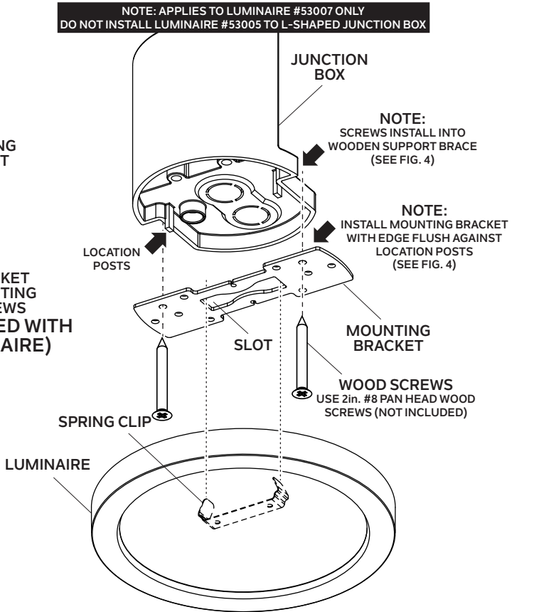
Fig. 3 INSTALLING TO L-SHAPED CEILING FAN JUNCTION BOX
