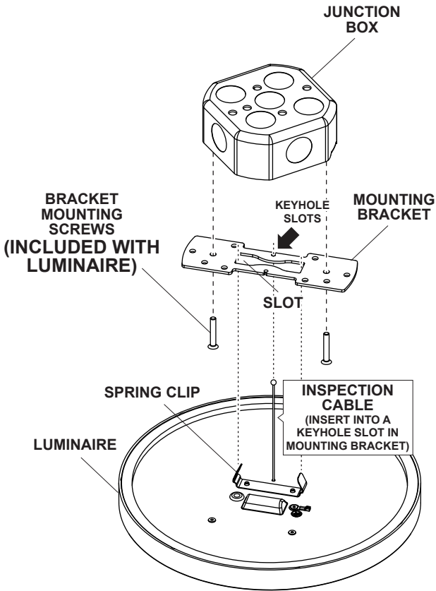
Fig. 1 INSTALLING TO STANDARD JUNCTION BOX
