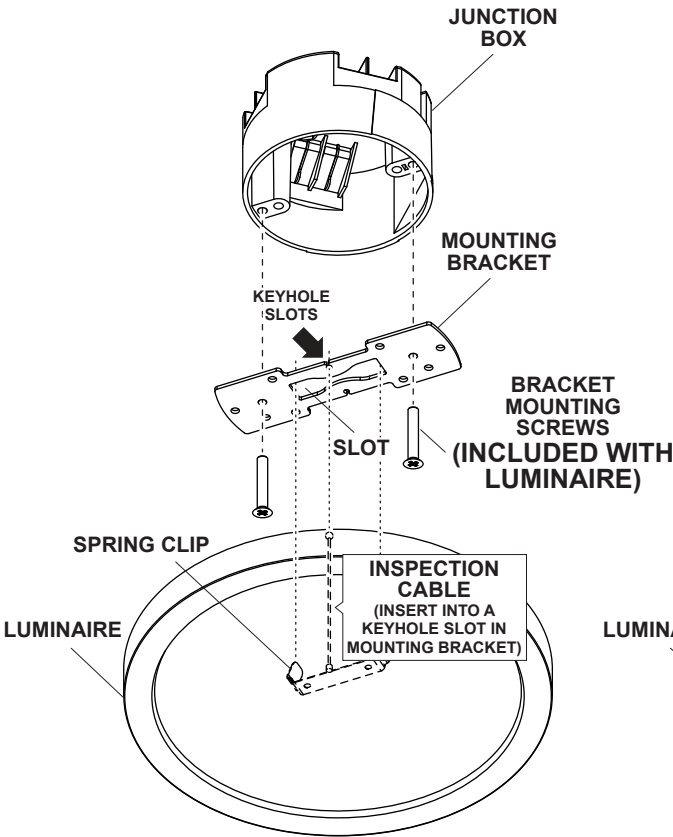
Fig. 2 INSTALLING TO ROUND CEILING FAN JUNCTION BOX
